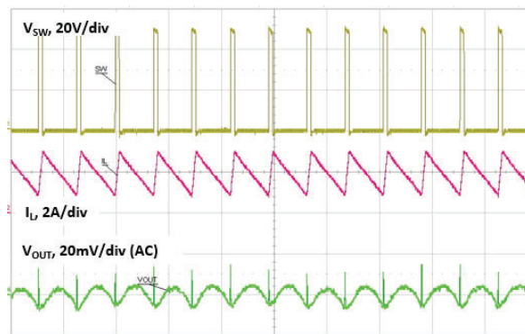
Fig. 29 - Output Ripple 2 A, Time = 5 \mu\text{s}/\text{div}
