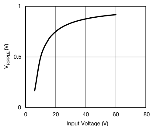
Fig. 7 - Amplitude for V_{OUT} = 5 V
