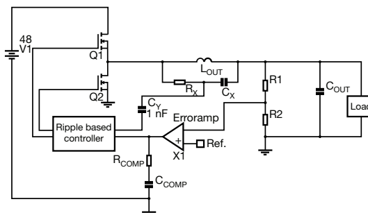
Fig. 5 - SiC46X Control Block Diagram
