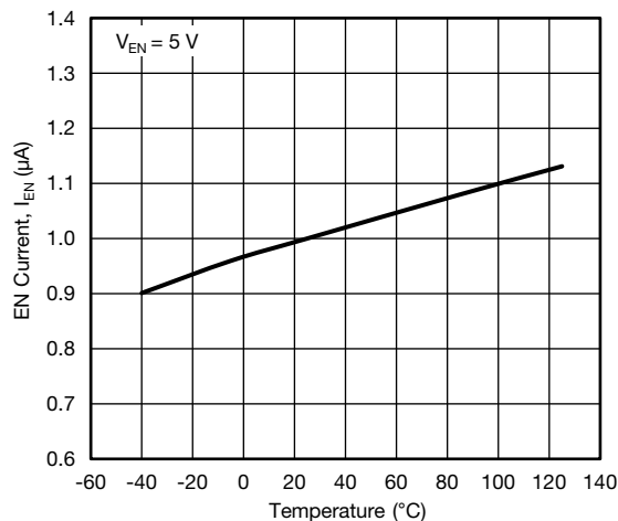
Fig. 23 - EN Current vs. Junction Temperature
