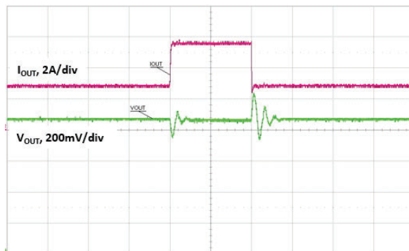
Fig. 27 - Load Transient (3 A to 6 A), (6 A to 3 A), Time = 100 \mu\text{s}/\text{div}
