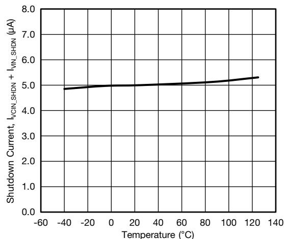
Fig. 21 - Shutdown Current vs. Junction Temperature
