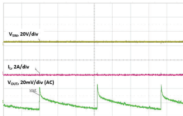
Fig. 31 - Output Ripple PSM, Time = 10 ms/div
