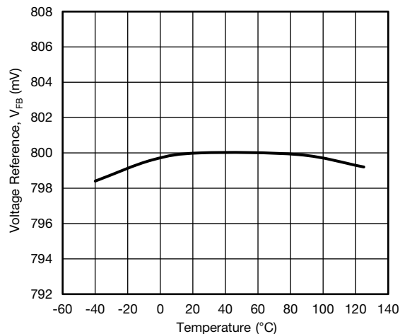
Fig. 24 - Voltage Reference vs. Junction Temperature
