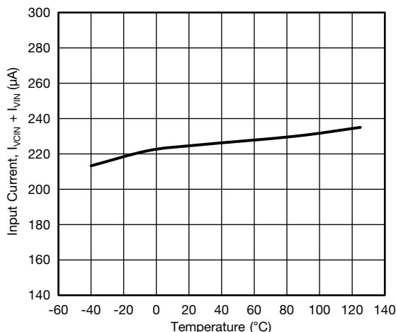
Fig. 17 - Input Current vs. Junction Temperature
