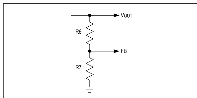
Figure 2. Adjusting Output Voltage
