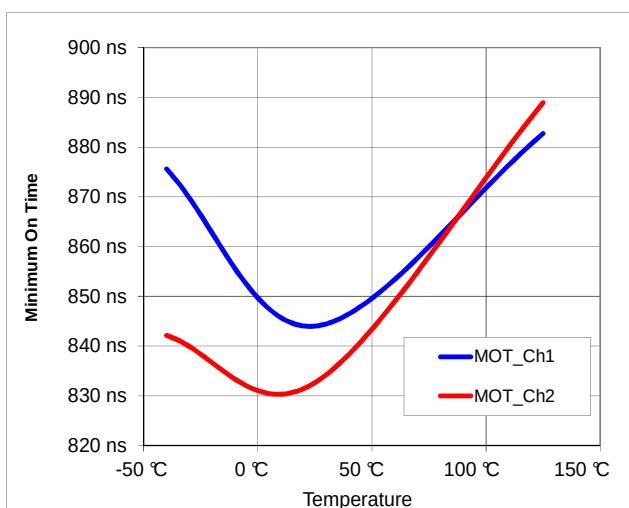
Figure 14: MOT vs Temperature
