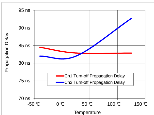
Figure 16: Turn-off Propagation Delay vs. Temperature
