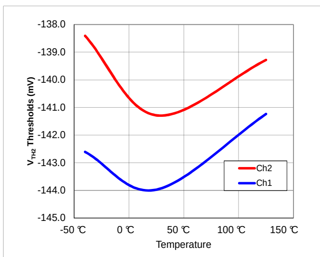
Figure 12: V_{TH2} vs. Temperature
